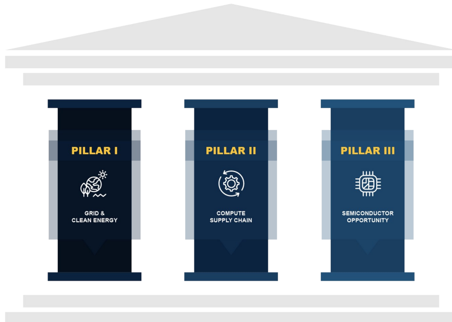
Figure 3. Three-Pillar Framework
